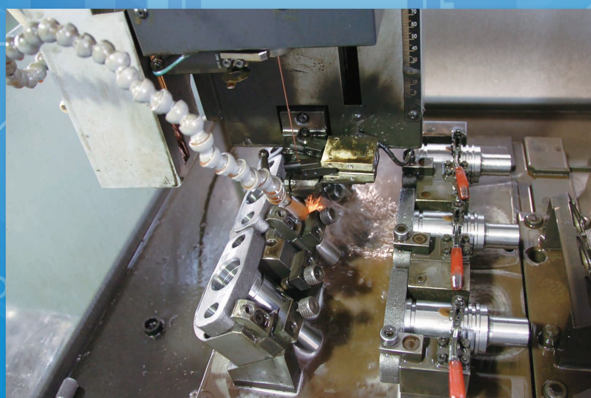
Electrical discharge machining
