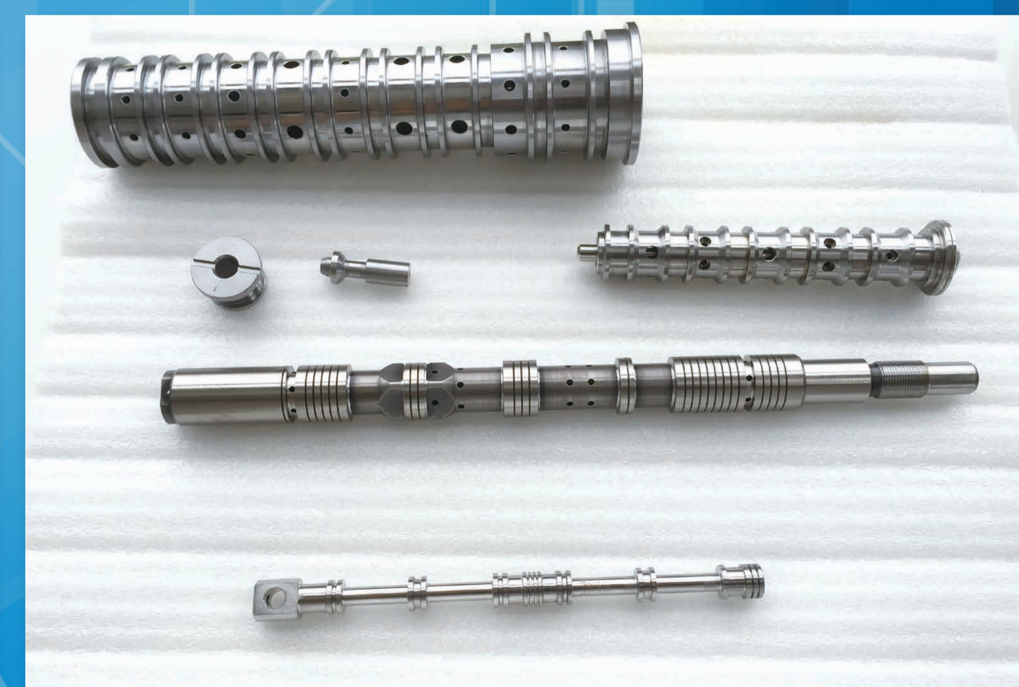
Hydraulic parts for Aircraft
